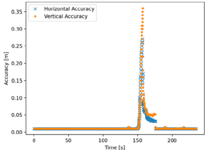
Figure 17: The effect of the tunnel on the horizontal and vertical accuracy of image positions.
