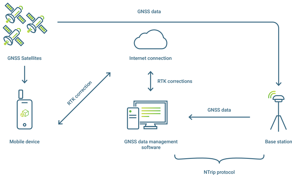
Figure 1: RTK device operation.
